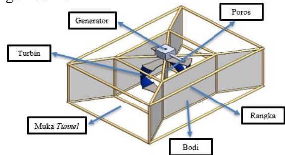
Gambar 2. Desain Tunnel Diffuser
