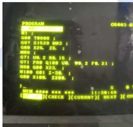
Gambar 4. 5 Program CNC
