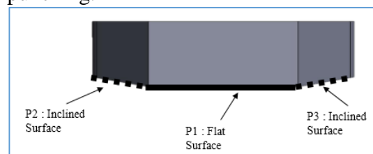
Figure 9. Design of punch shapes
